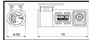
Dimension of Main Camera (mm)
